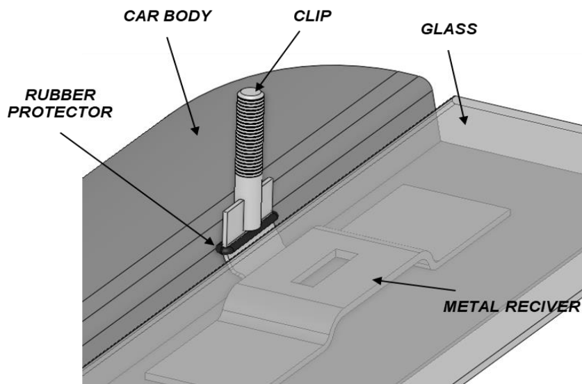
INSIDE RECIVER Correct fitting
